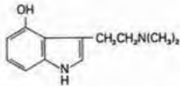
PSILOCIN
